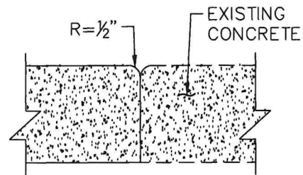
CONSTRUCTION JOINT
