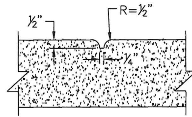
SCORE LINE
