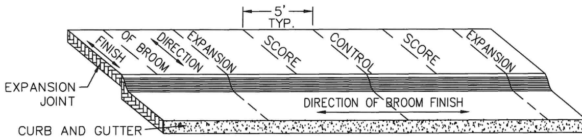
SIDEWALK FINISH
